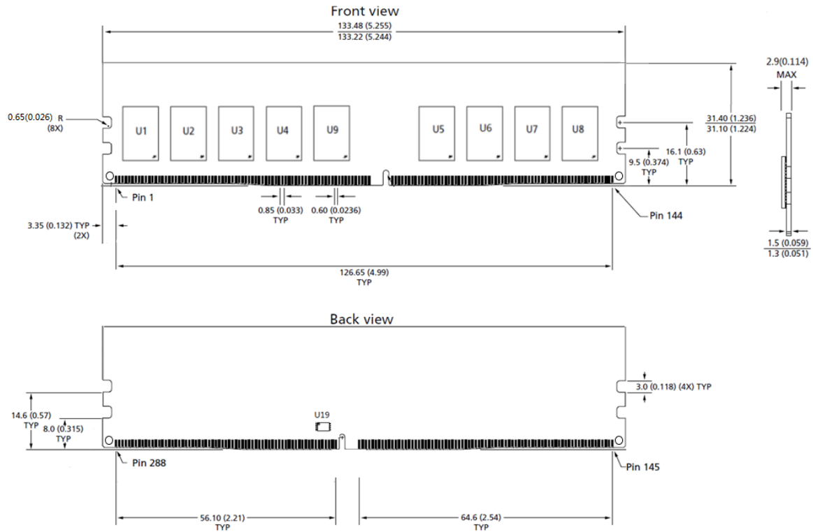
Figure 3 – Package Dimensions_SCC16GE03H4F1C-32AA
