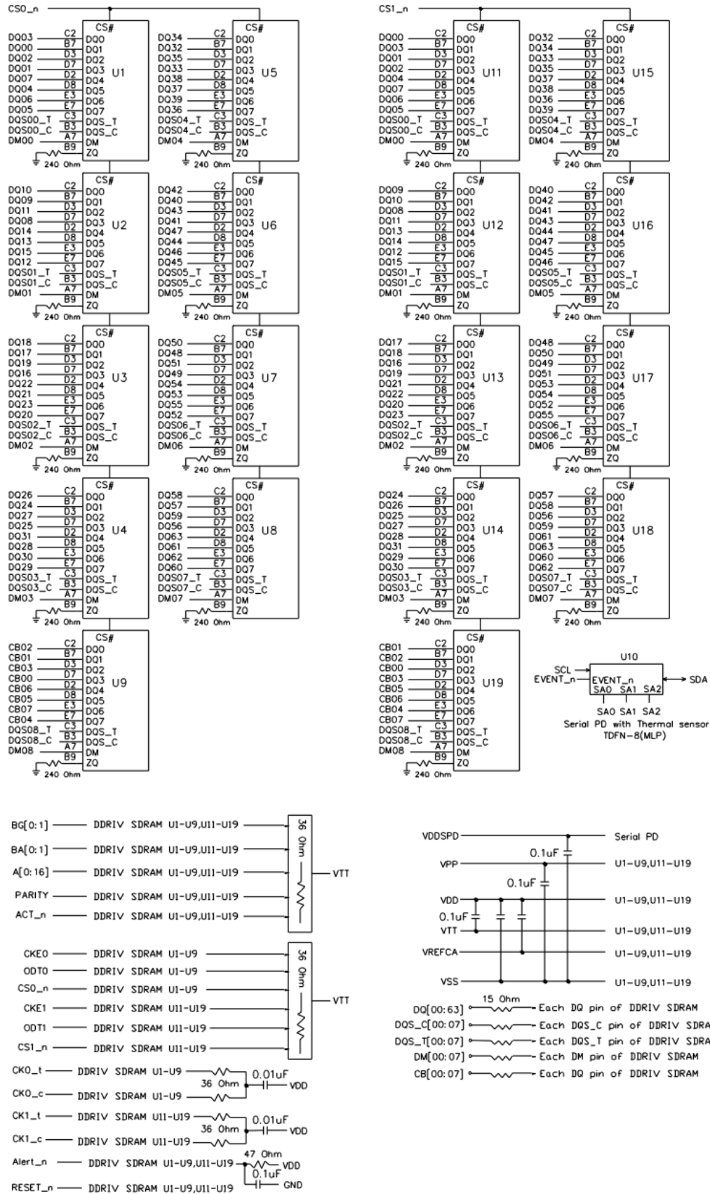
Figure 2 – Function Block Diagram_SCC32GE13H4F1C-32AA
