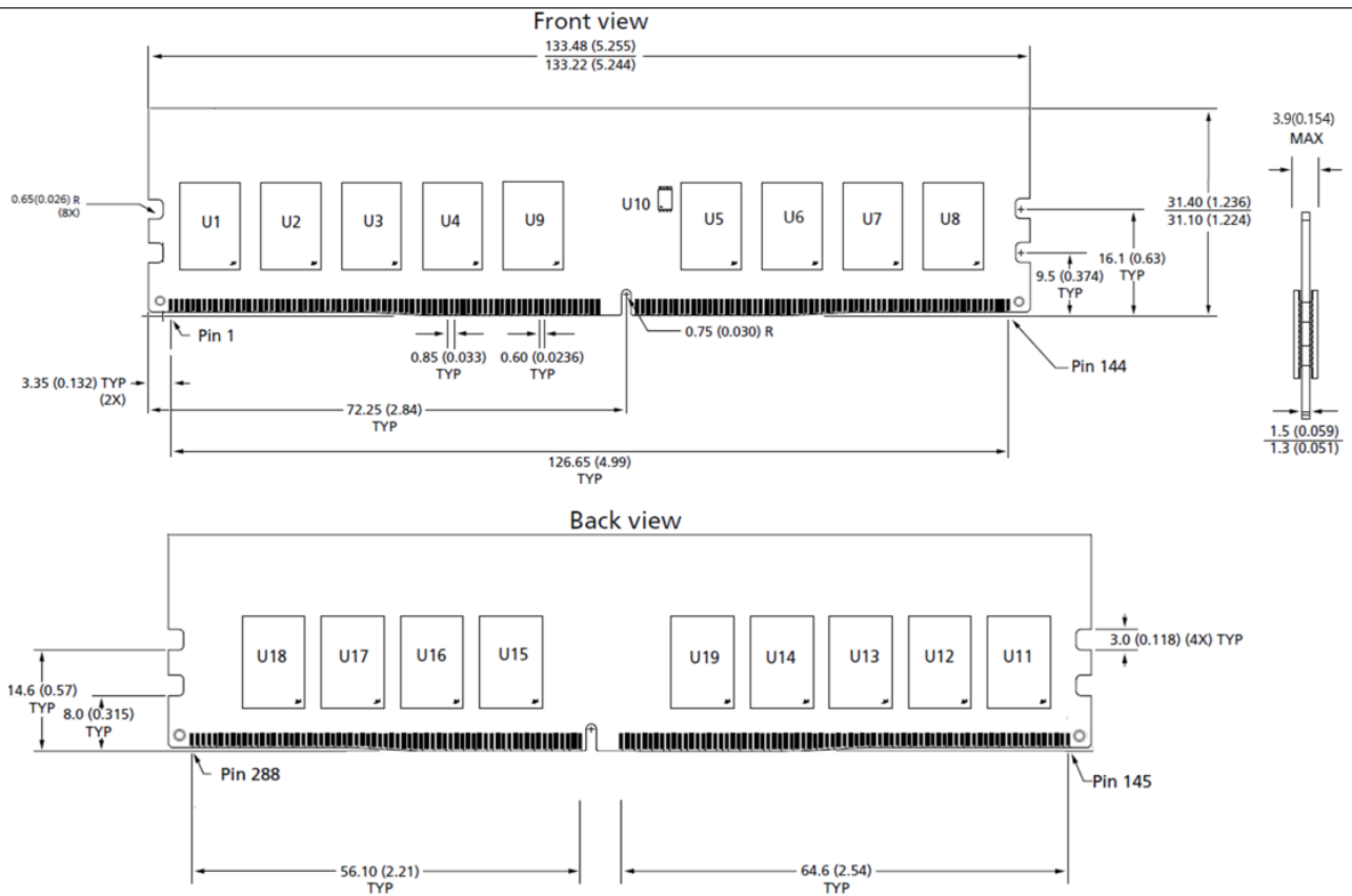
Figure 4 – Package Dimensions_SCC32GE13H4F1C-32AA
