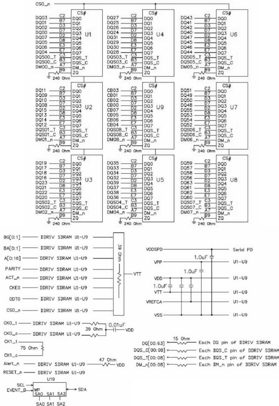
Figure 1 – Function Block Diagram_SCC16GE03H4F1C-32AA
